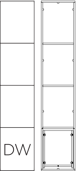
Three Door Locker and One Drawer
