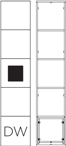
Four Door Locker and One Drawer with cut out for Smarty Terminal
